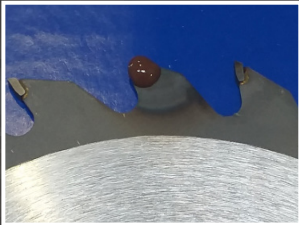
Application of CleanTech X85 Flux Paste
